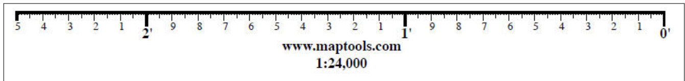
Figure 9.22. A Lat/Long ruler for a 7.5' Topo map (not to scale)
