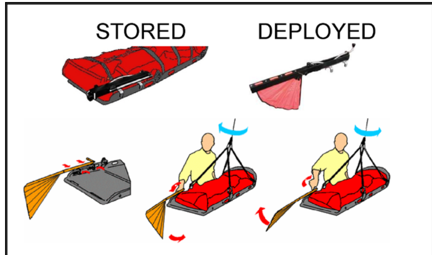
Figure 31- Anti-Rotation Stabilizer for helicopter hoisting attached to Franco Garda Stretcher. Images copyright TSL Rescue, France.
